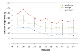
Fig. 5. Service Outage Times in the Function of the Delay from the Last C-RP-Adv Message to the Stopping of the RP on xorp2 Router
